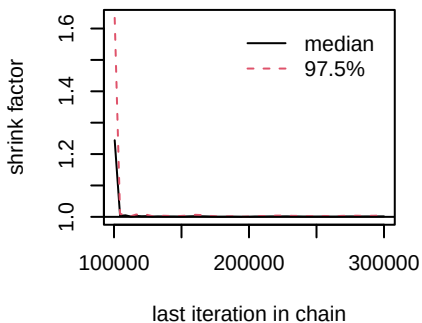
d.chemo.Afatinib
